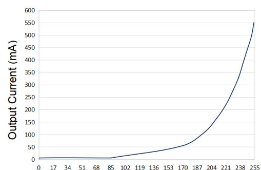
Logarithmic dimming
