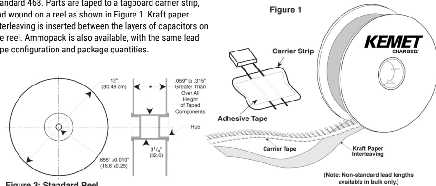
Figure 3: Standard Reel
