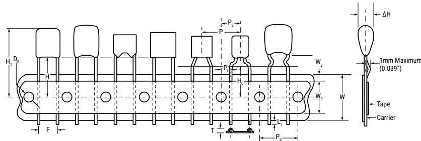
Figure 2: Lead Tape Configuration (See Table Below)
