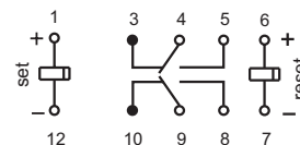
reset condition
