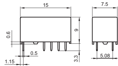
2 coils latching
