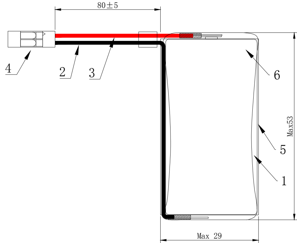
Dupont.DB2.54 connector
