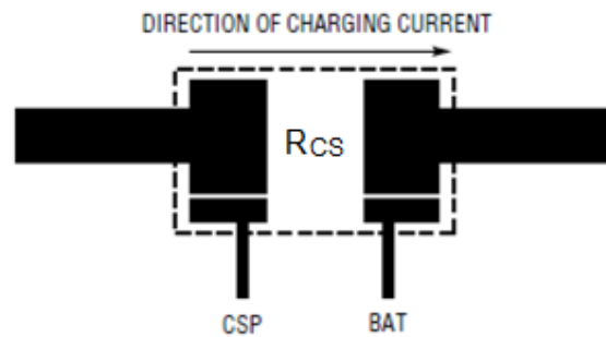
Figure 4 Kelvin Sensing of Charge Current
