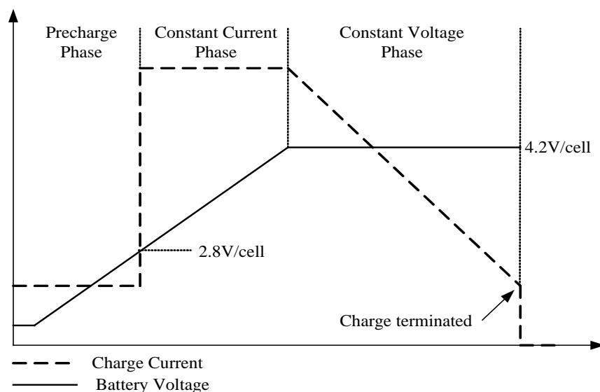
Figure 2 The Charging Profile
