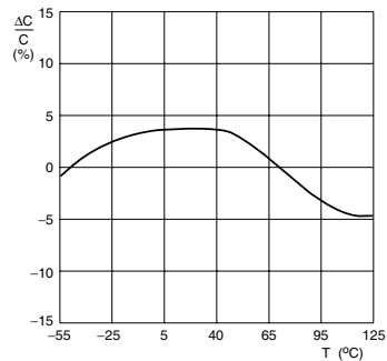
Fig. 4 Typical capacitance change as a function of temperature
