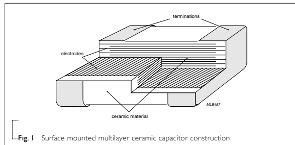
Fig. 1 Surface mounted multilayer ceramic capacitor construction
