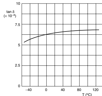
Fig. 3 Typical tan \delta as a function of temperature
