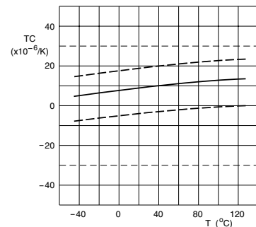
Fig. 2 Typical temperature coefficient as a function of temperature
