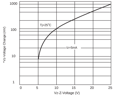
Figure 2. Typical Change of Working Voltage under Operating Conditions at Tamb=25°C
