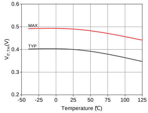
Figure 22: V_{IT,TH-} vs. temperature
