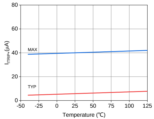
Figure 12: I_{TRIP+} vs. temperature
