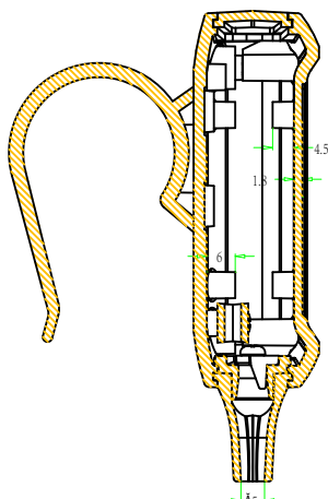
SEC B-B
