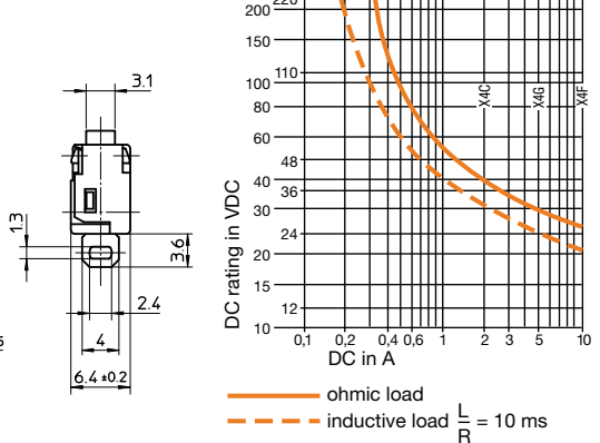
Maximum DC rating
