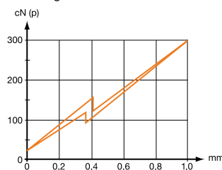
Actuating force/travel
