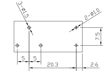
TRC1 D-xxVDC-S-x 2
