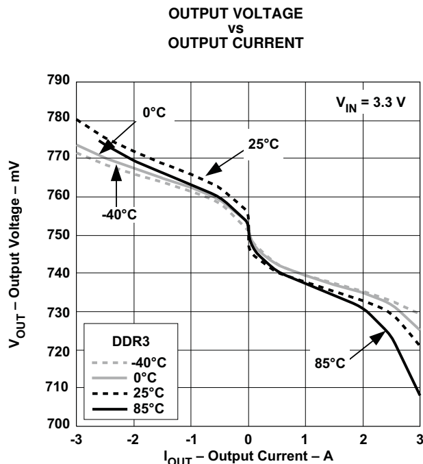
Figure 6. DC Regulation
