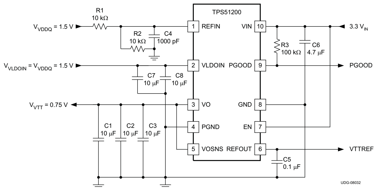
Figure 29. 3.3\text{-V}_{\text{IN}} , DDR3 Tracking Configuration
