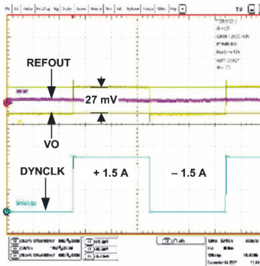
Figure 7. Transient
