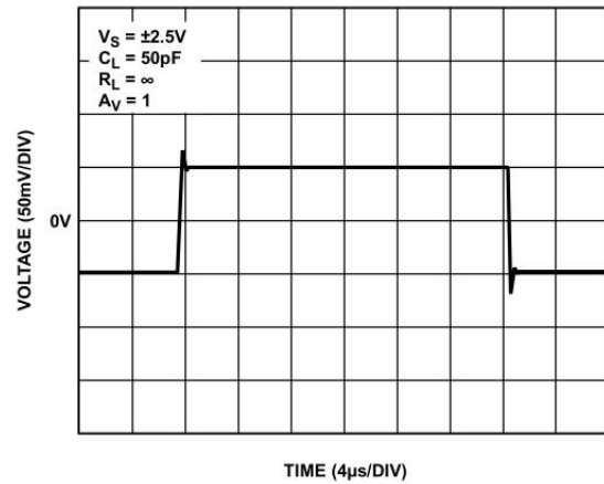
Figure 8. Small Signal Transient Response
