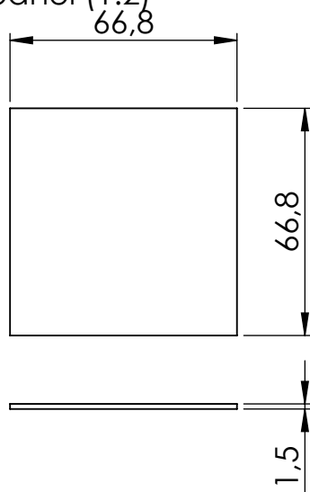
Front panel (1:2)
