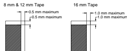
Figure 3 – Maximum Lateral Movement
