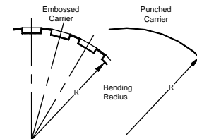
Figure 4 – Bending Radius
