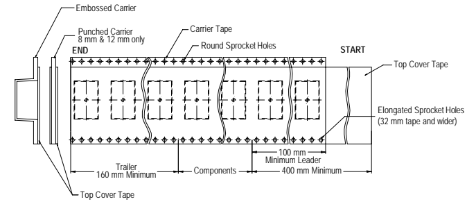
Figure 6 – Tape Leader & Trailer Dimensions
