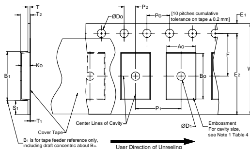
Figure 1 – Embossed (Plastic) Carrier Tape Dimensions
