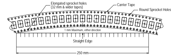
Figure 7 – Maximum Camber
