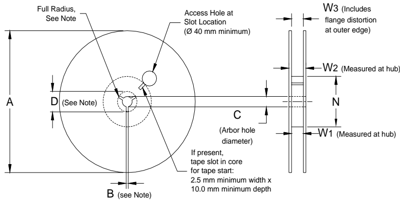
Figure 5 – Reel Dimensions
