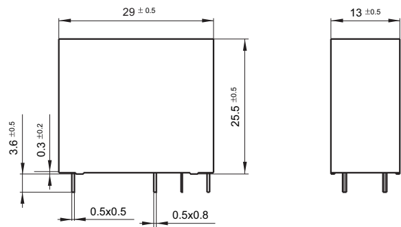
Outline Dimensions
