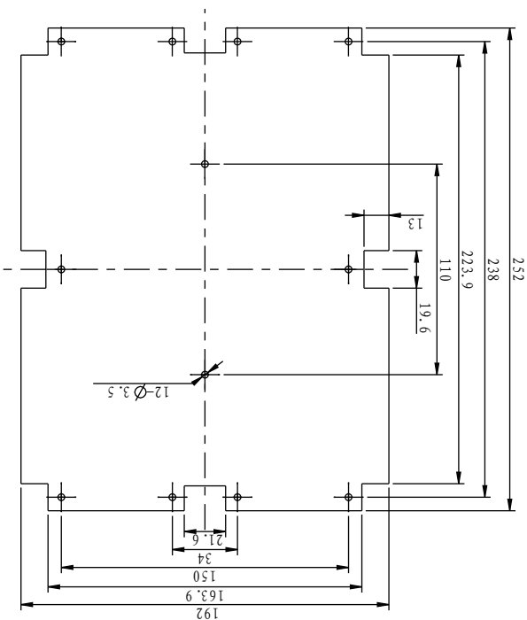
PCB
